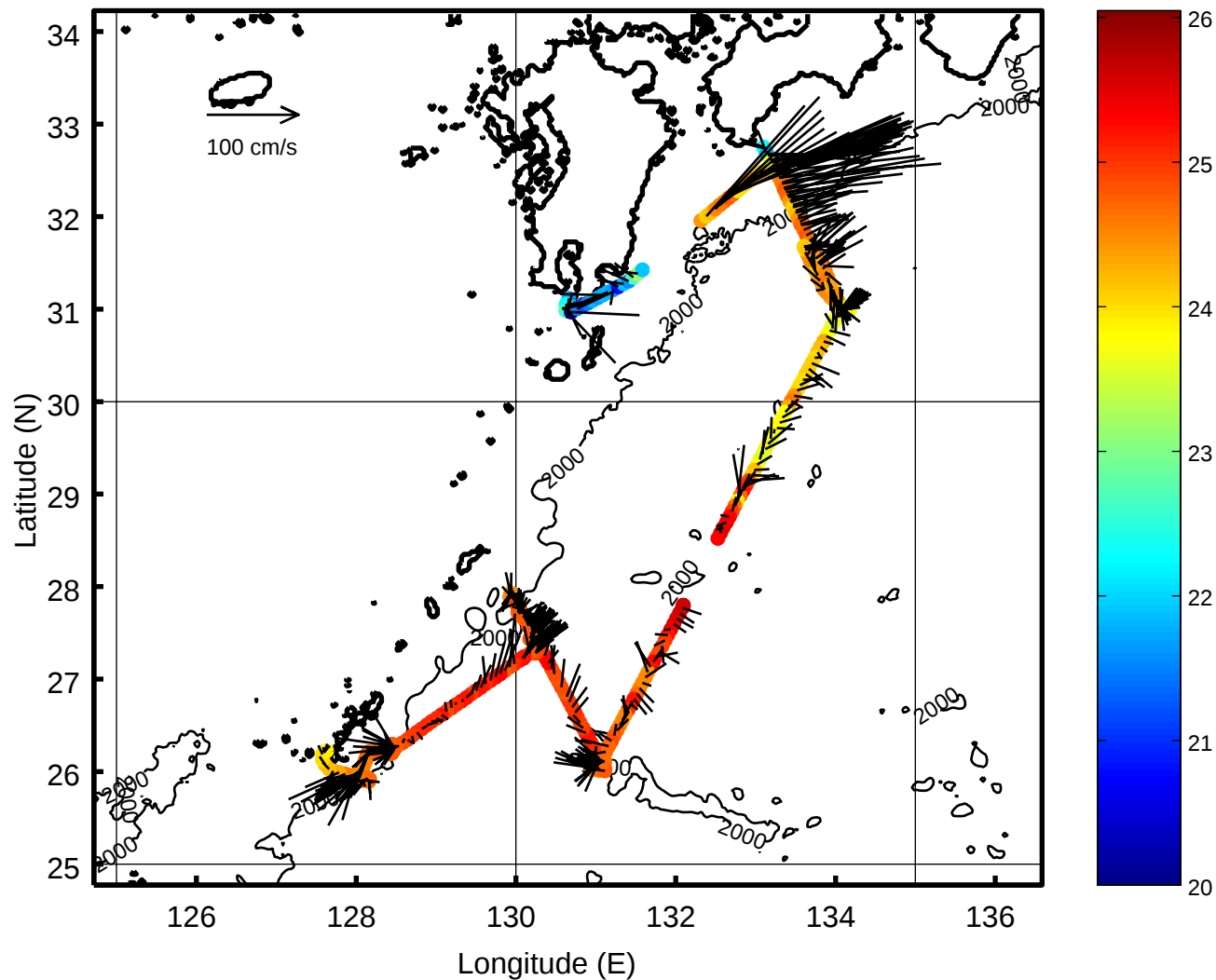
SST and SSC in Nov.14-24, 2001
