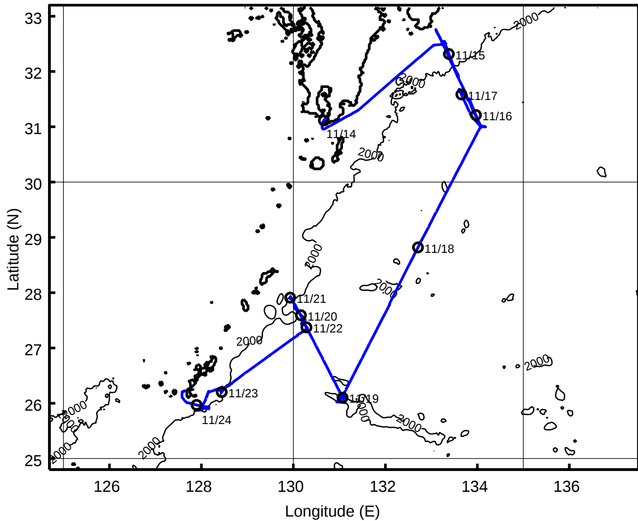
Ship's Track in KE01-19 Cruise
