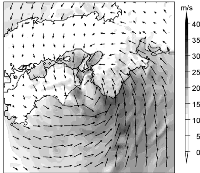
Figure 6. Distribution of the horizontal wind vectors from the lowest layer in Domain 2, approximately 11 m above the ground surface. 1330 LST, 22 September, 1998.
