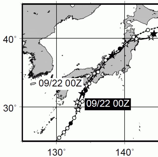
Figure 4. Comparison between the simulated data (☆) and JMA best track data (○): trajectory of the location of the lowest pressure in Typhoon No. 9807.
