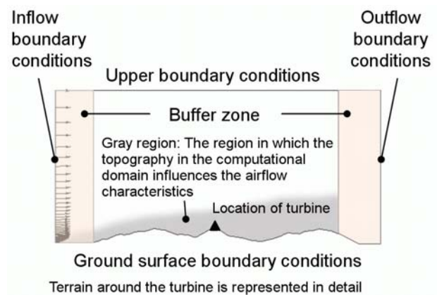
Figure 7. Boundary conditions used in the RIAM-COMPACT ® CFD model.
