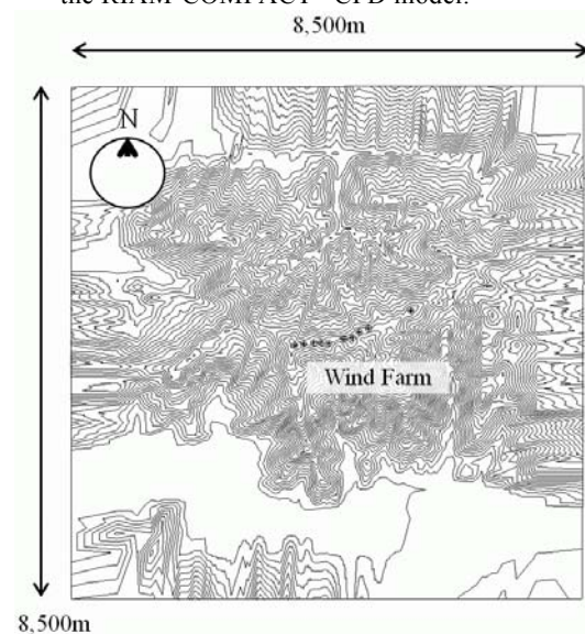
Figure 8. Computational domain used in the RIAM-COMPACT ® CFD model.
